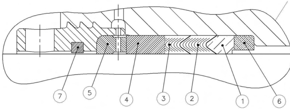
CDI PACKING ASSEMBLY DETAIL 4” CDI PACKING ASSEMBLY*
