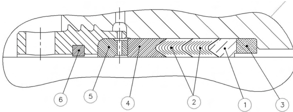
RSL PACKING ASSEMBLY DETAIL
